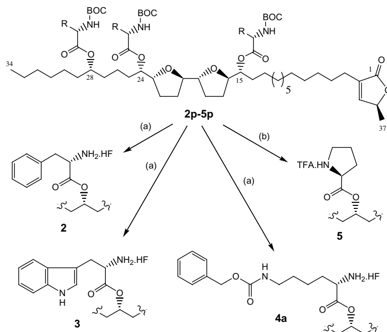
Scheme 2. Deprotection of the N α -BOC groups of the triesters 2p-5p . Reagents and conditions: (a) 2p-4p , HF/Py, anisole, 0 °C to rt, 2 h (68% 2 , 39% 3 , 57% 4a ); (b) 5p , TFA, CH 2 Cl 2 , 0 °C, 2 h (55%).
