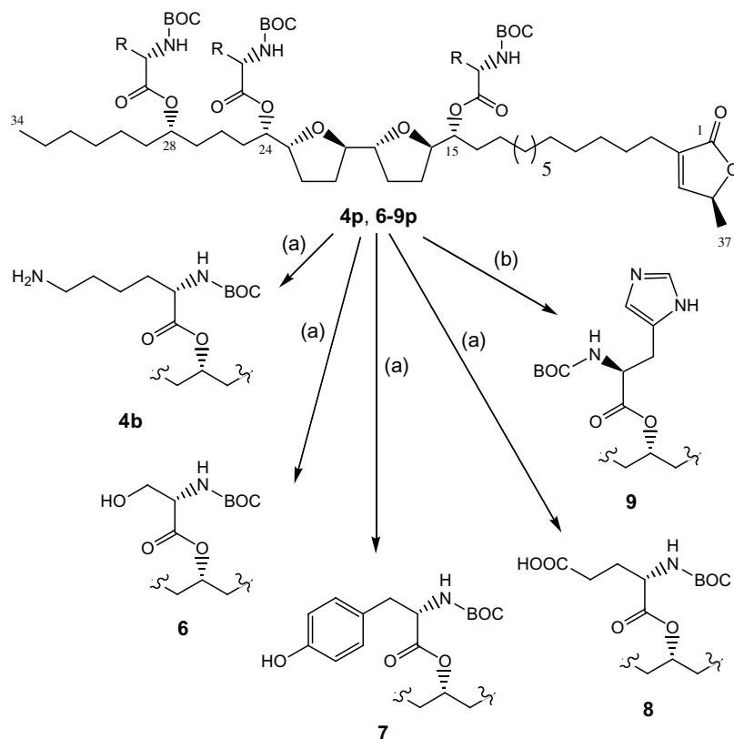
Scheme 3. Deprotection of the lateral chains of triesters 4p and 6p–9p . Reagents and conditions: (a) 4p , 6–8p , Pd–C (10%), 1,4-cyclohexadiene, EtOH, 40–65 °C, 2–8 h (86% 4b , 52% 6 , 60% 7 , 32% 8 ); (b) 9p , HOBT, THF, rt, 5 h (42%).
